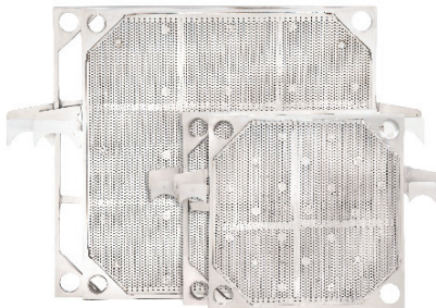
(Gasketless Design)
